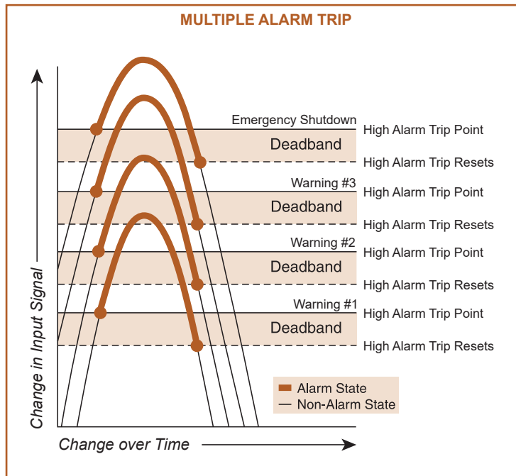
Figure 6. Alarm trips with multiple relays can be configured to provide various levels of protection such as Warning #1, Warning #2, Warning #3 and ultimately Emergency Shutdown.
