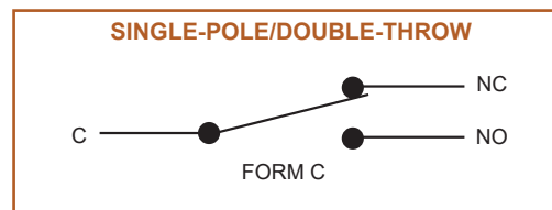
Figure 12. Single-Pole/Double-Throw (SPDT) relay contacts are shown with the de-energized (shelf) state.
