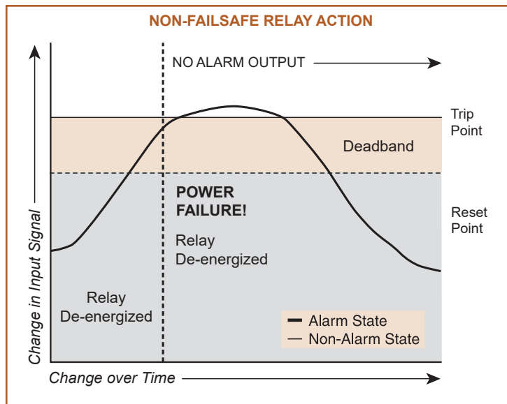
Figure 15. Non-Failsafe Relay Action upon power failure.
