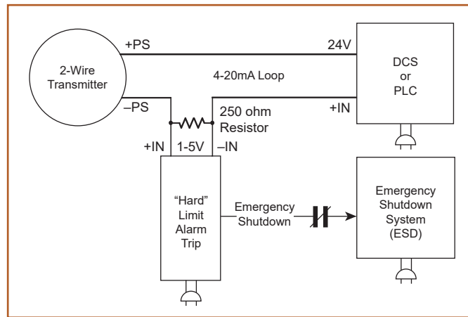
Figure 2. Since “Hard” alarms are isolated and independent, they are not susceptible to common-mode failure issues that arise in the PLC or DCS system.
