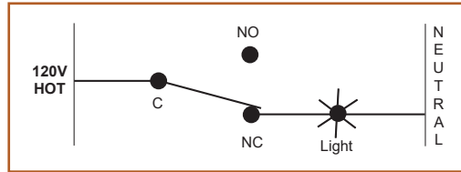
Figure 17. A failsafe alarm trip is energized when it is not in the alarm state and de-energized when in alarm state.
