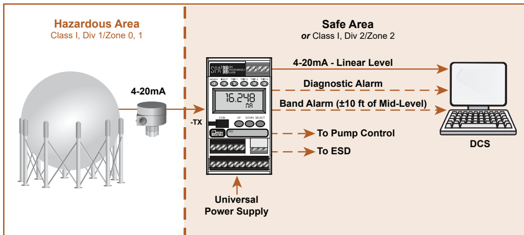
Figure 22. An associated apparatus incorporating a spherical tank linearization measurement function, local pump control, Hi-Hi ESD, local indication, self diagnostics and quad relay outputs for control and alarming.
