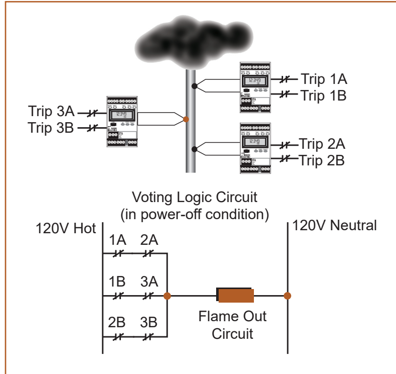
Figure 23. Alarm trips in a 2oo3 voting scheme.
