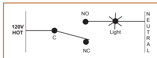
Figure 16. A non-failsafe alarm is de-energized when in normal state (shown below) and energized when in alarm state.
