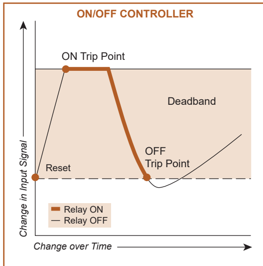
Figure 10. On/Off Control.
