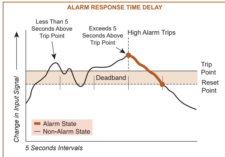
Figure 19. Alarm time delay stops false or premature alarms.
