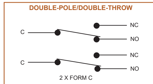
Figure 13. Double-Pole/Double-Throw (DPDT) relay in the energized state.
