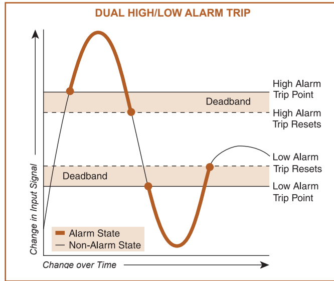
Figure 1. Limit alarm trips monitor a process signal and send one or more relay outputs when a monitored signal exceeds preset high and/or low limits (dual high/low alarm configuration shown).
