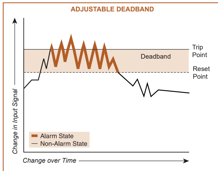
Figure 18. Deadband reduces relay chatter.
