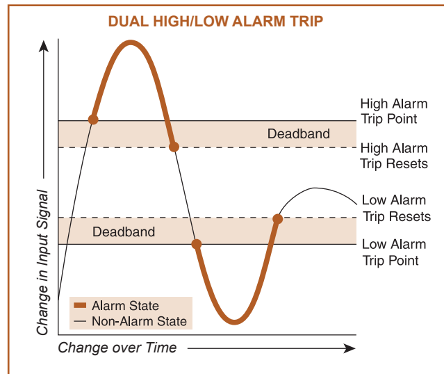
Figure 4. Dual high/low limit alarm trip with deadband to reduce relay chatter.
