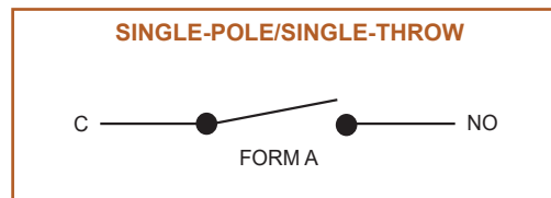
Figure 11. Single-Pole/Single-Throw (SPST) Relay shown with a normally-open (NO) contact in the de-energized (shelf) state.
