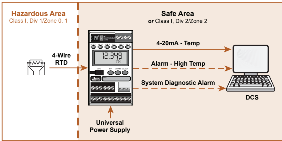
Figure 21. An associated apparatus incorporating the isolating barrier, temperature transmitter, temperature alarm and diagnostic alarming functions in a single device.
