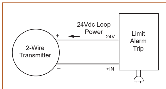
Figure 20. Alarm trip providing 24Vdc power to the loop.
