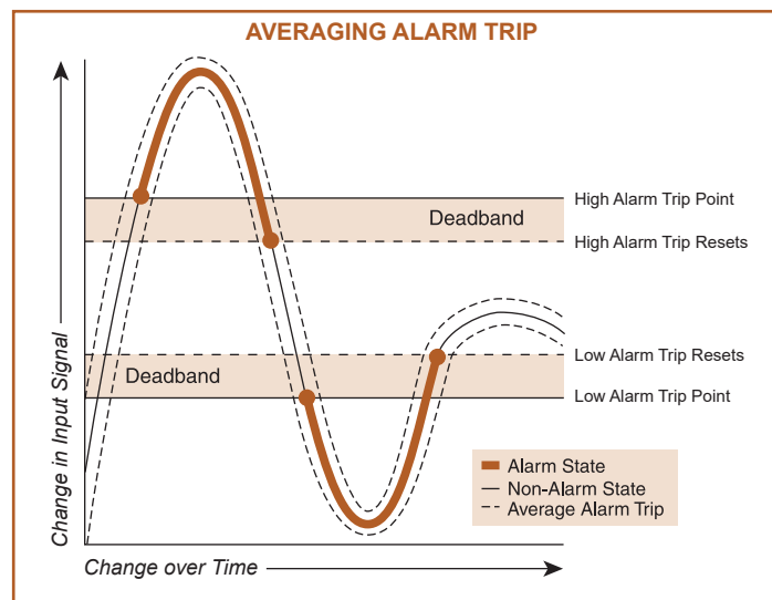
Figure 8. Averaging Alarm Trip.
