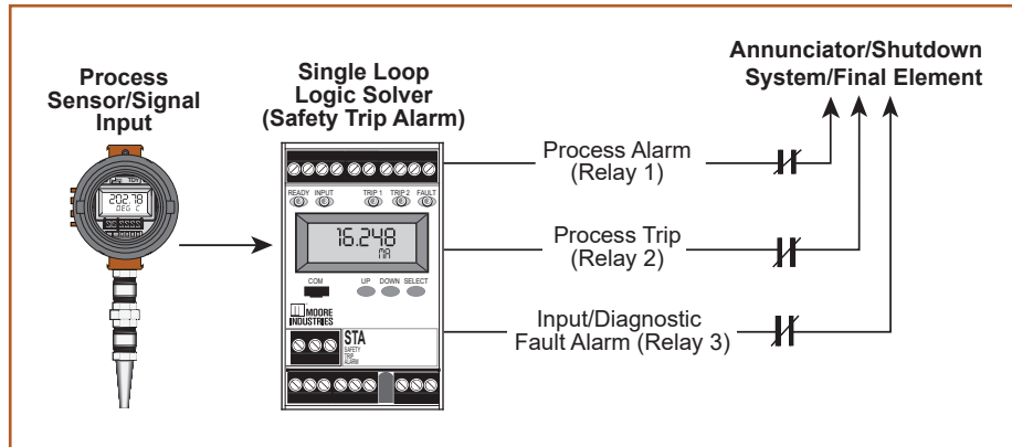
Figure 3. A typical Safety Instrumented System (SIS) is comprised of any number or combination of sensors, logic solvers and final control elements.
