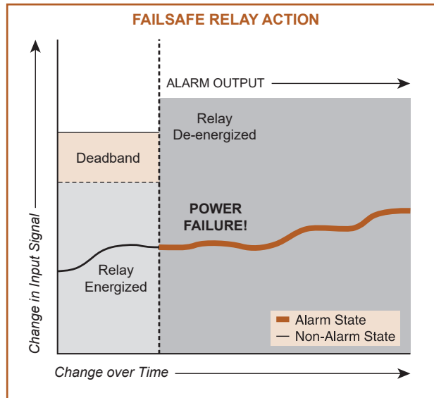
Figure 14. Failsafe Relay Action upon power failure.
